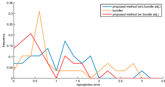
Figure 10. The reprojection error distribution for real data (Capitol sequence) using only two point-tangents, before and after bundle adjustment.
