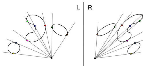
Figure 4. Correspondence of epipolar tangencies used in curve-based camera calibration. An epipolar line on the left, whose tangency at a curve is marked in a certain color, must correspond to the epipolar line on the right having tangency on the corresponding curve, marked with the same color. This concept works for both static curves and occluding contours.
