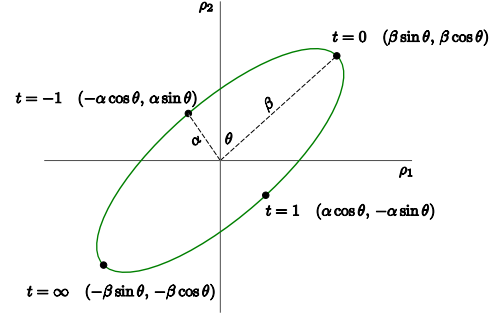
Figure 7. Diagram illustrating a parametrization of the ellipse by a parameter t .
