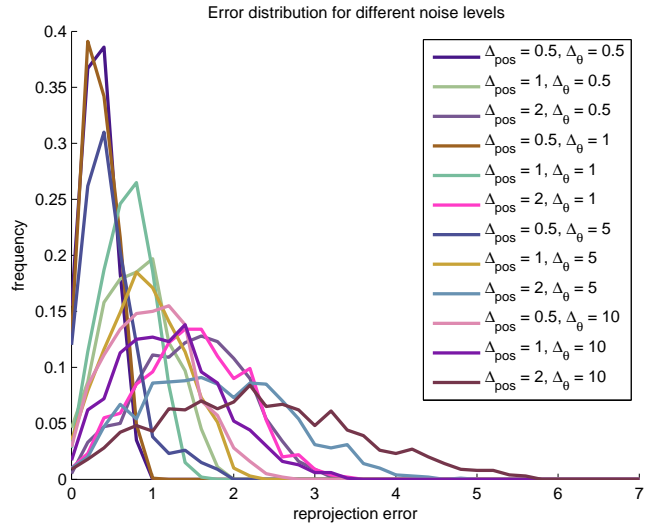
Figure 9. Distributions of reprojection error without running bundle adjustment, for increasing levels of positional and tangential perturbation in the measurements.
