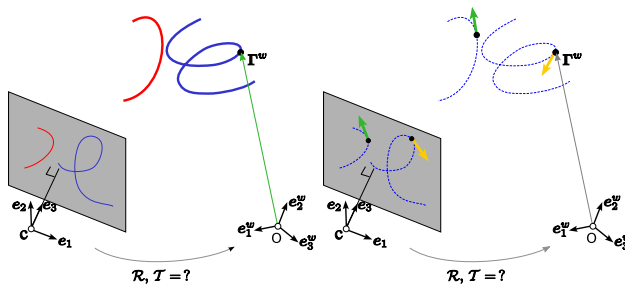
Figure 3. The problem of finding the camera pose \mathcal{R}, \mathcal{T} given space curves in a world coordinate system and their projections in an image coordinate system (left), and an approach to that consisting of (right) finding the camera pose \mathcal{R}, \mathcal{T} given 3D point-tangents (i.e., local curve models) in a world coordinate system and their projections in an image coordinate system.
