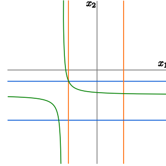
Figure 6. Diagram of the mutual intersection of Equations 3.2–3.4 in the x_1 – x_2 plane.
